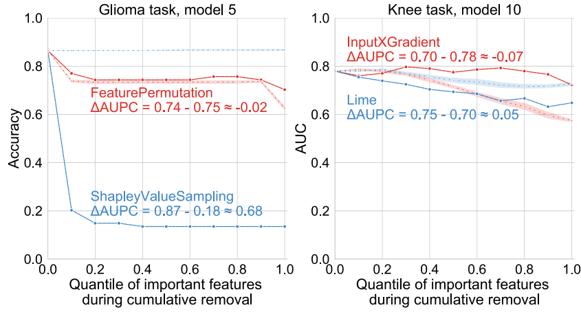
Fig. 3. Feature perturbation curves for the cumulative feature removal experiment. Feature perturbation curves in solid line are the model performance deterioration for an XAI method \mathcal{H} , and curves in dashed line are the XAI method counterpart baselines \mathcal{H}_b of random feature removal. The random baseline experiment was repeated 15 times, thus the dashed line also has its 95% confidence interval as translucent error band. We show plots of the XAI method that has the highest (blue) and lowest \Delta\text{AUPC} score (red curve) from a model for both clinical tasks. \text{AUPC}(\mathcal{H}_b) and \text{AUPC}(\mathcal{H}) which are used in the calculation of \Delta\text{AUPC} are also indicated on the plot for each XAI method: \Delta\text{AUPC} = \text{AUPC}(\mathcal{H}_b) - \text{AUPC}(\mathcal{H}) . Numbers reported in the subtraction are rounded to two decimal places.
