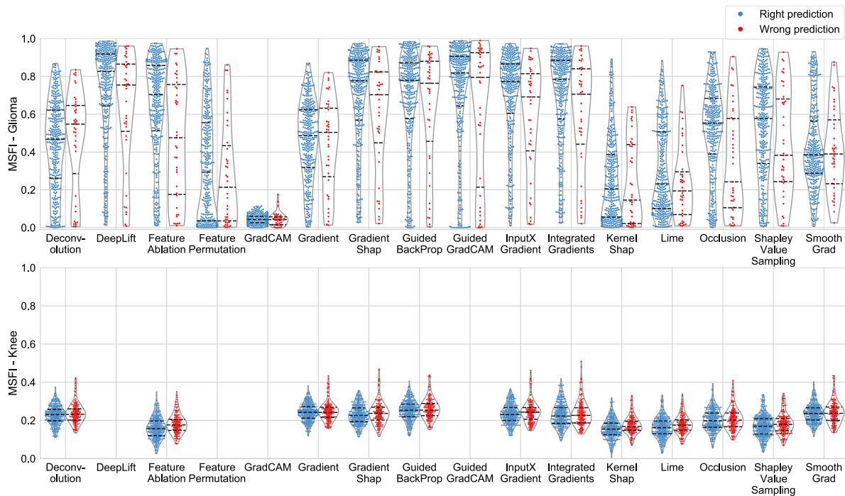
Fig. 5. Evaluation results on Guideline 4 – Testing for plausibility informativeness. For each heatmap method ( X -axis), the violin and swarm plots show the plausibility quantification score distribution of MSFI for the right (blue, left) and wrong (red, right) predictions on the glioma (top) and knee task (bottom). Each dot is a data sample in the test set, and we aggregate results from five similarly-trained models. Y -axis is the MSFI measure, with a higher score indicating more agreeable of a heatmap with clinical prior knowledge on modality prioritization and feature localization. The black dashed lines indicate the quartiles of each distribution.
